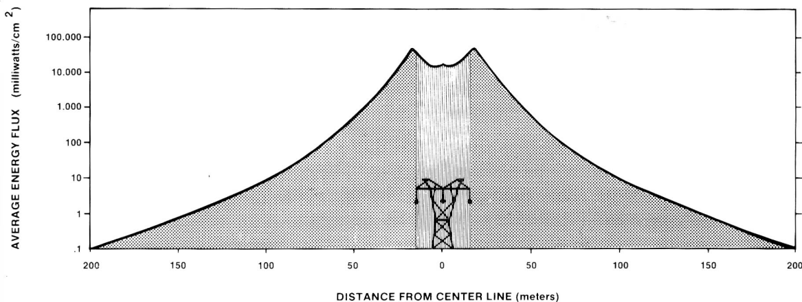
Figure 1: Average ground-level energy flux associated with a typical 765 kV powerline as a function of lateral distance from the center line of the powerline.
